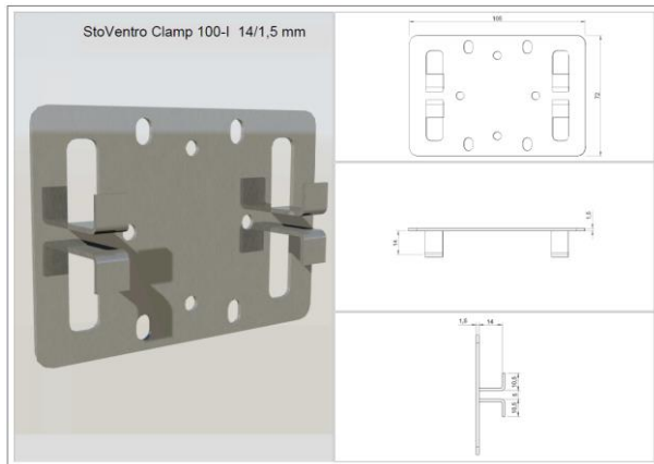
StoVentro Clamp 100-I 14/1.5 mm
