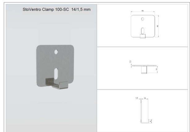
StoVentro Clamp 100-SC 14/1.5 mm
