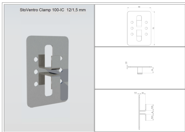
StoVentro Clamp 100-IC 12/1.5 mm
