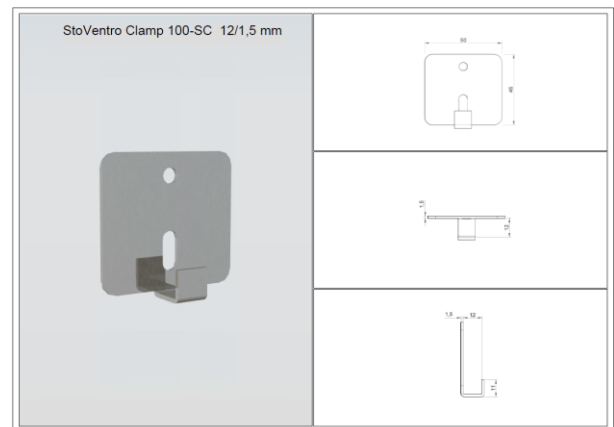
StoVentro Clamp 100-SC 12/1.5 mm
