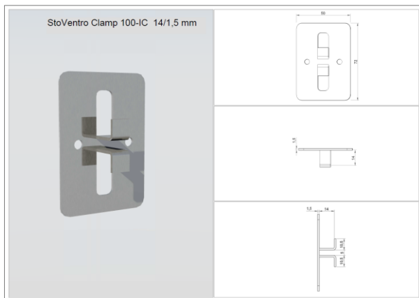
StoVentro Clamp 100-IC 14/1.5 mm
