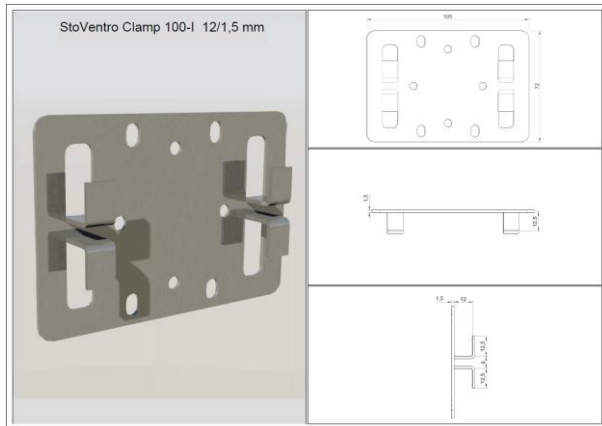
StoVentro Clamp 100-I 12/1.5 mm
