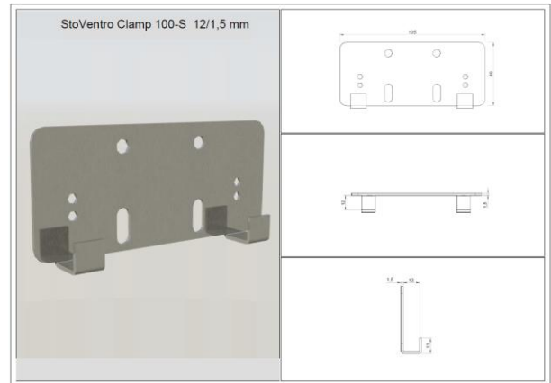
StoVentro Clamp 100-S 12/1.5 mm
