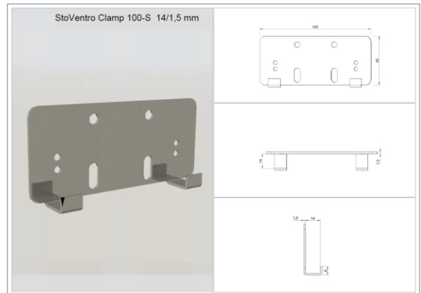
StoVentro Clamp 100-S 14/1.5 mm
