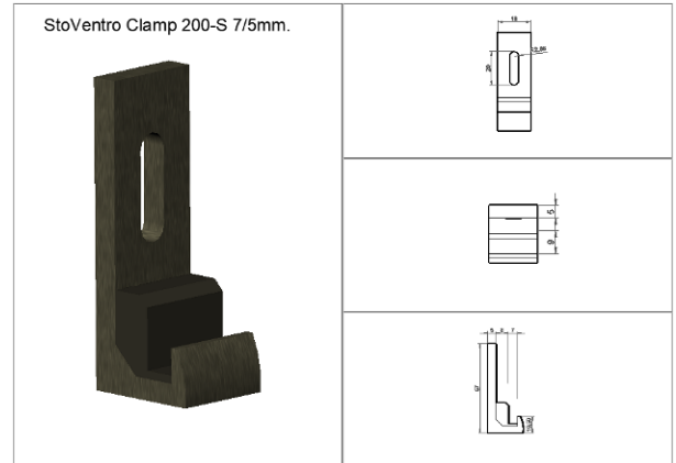
StoVentro Clamp 200-S 7/5mm
