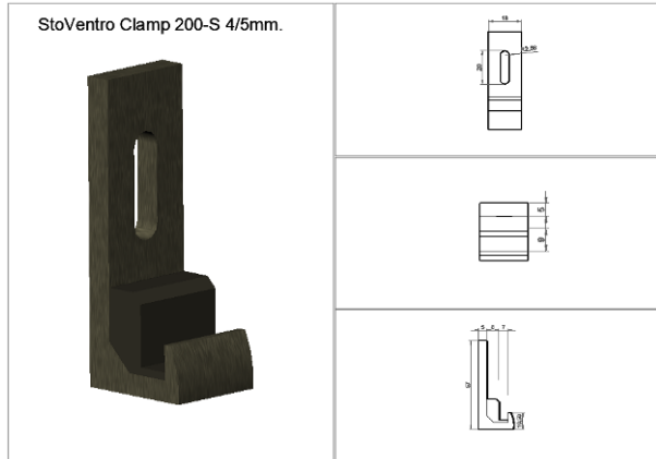
StoVentro Clamp 200-S 4/5mm
