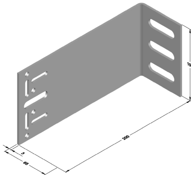
StoVentro Bracket L201 DFP
