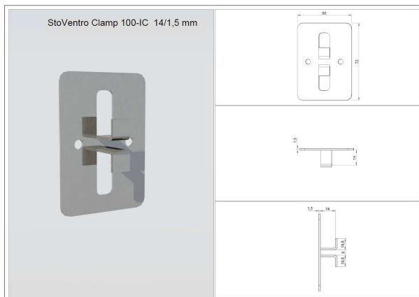
StoVentre Clamp 100-IC 14/1.5 mm
