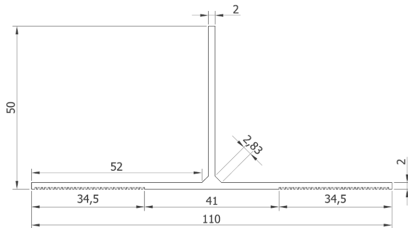
StoVento Profile T202
