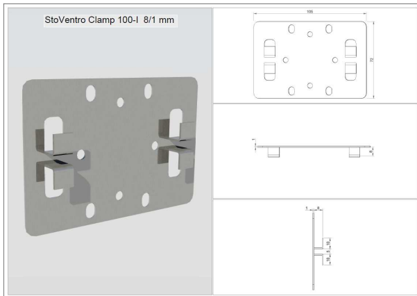
StoVento Clamp 100-I 8/1 mm
