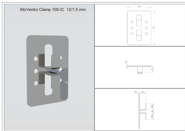
StoVentre Clamp 100-IC 12/1.5 mm
