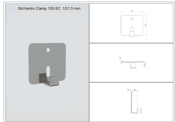
StoVentre Clamp 100-SC 12/1.5 mm
