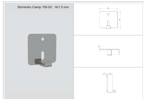
StoVentre Clamp 100-SC 14/1.5 mm
