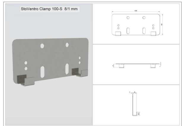
StoVento Clamp 100-S 8/1 mm
