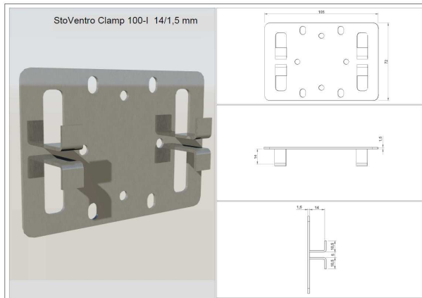
StoVentre Clamp 100-I 14/1.5 mm
