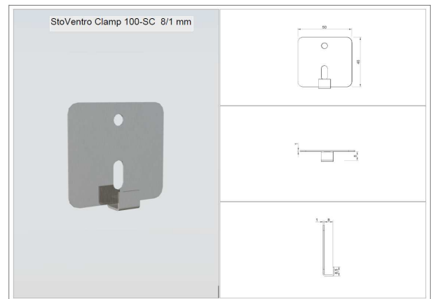
StoVento Clamp 100-SC 8/1 mm
