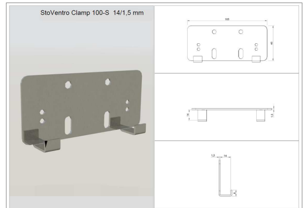
StoVentre Clamp 100-S 14/1.5 mm
