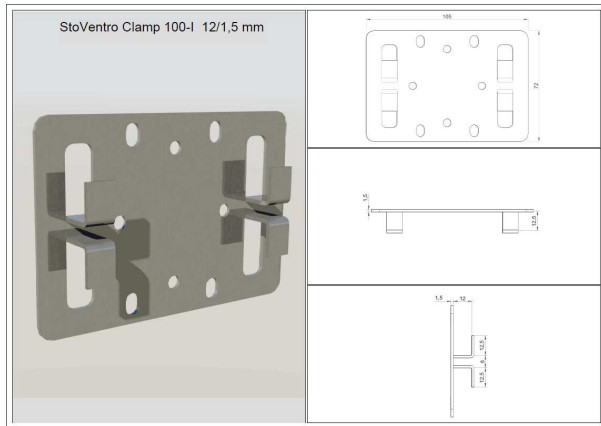
StoVentre Clamp 100-I 12/1.5 mm
