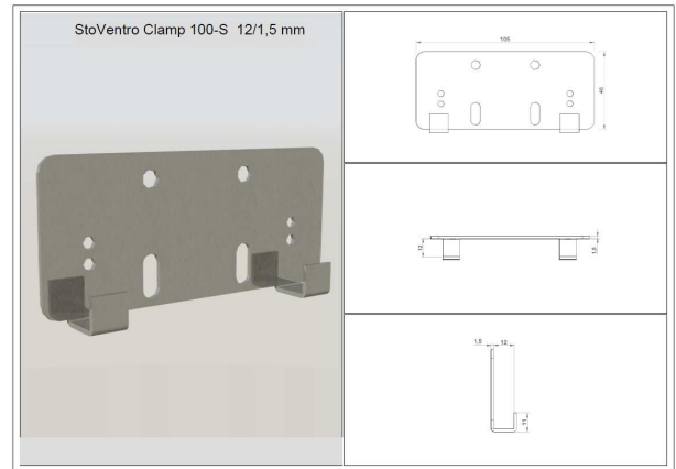
StoVentre Clamp 100-S 12/1.5 mm
