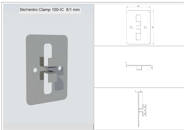
StoVento Clamp 100-IC 8/1 mm
