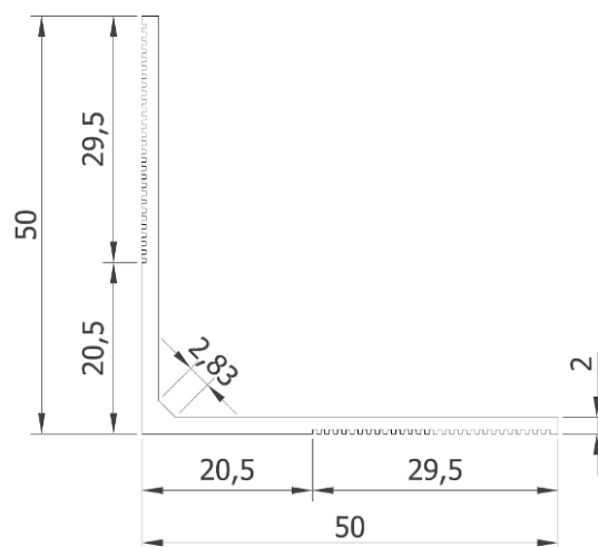
StoVento Profile L202
