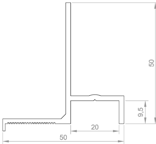
StoVento Profile L204
