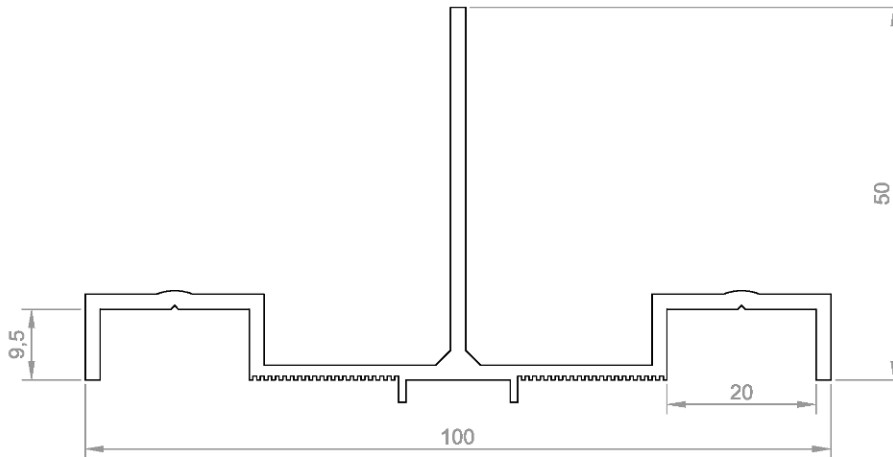
StoVento Profile T204
